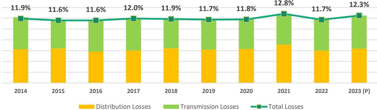
Figure 2: System Losses
